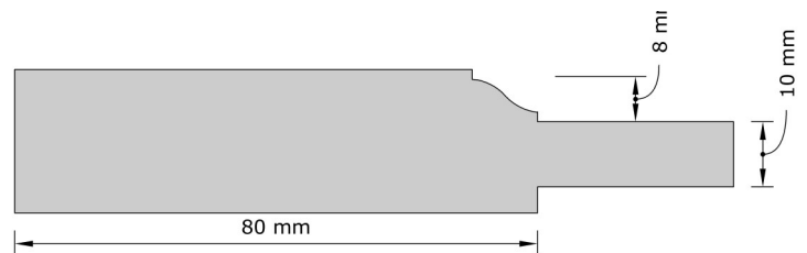
OGEE
